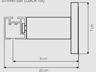
8.0 cm wall bracket universal (back fix)
