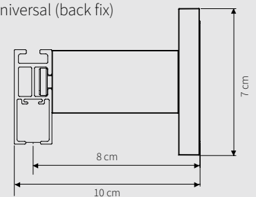
8.0 cm wall bracket universal (back fix)
