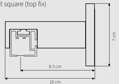
8.0 cm wall bracket square (top fix)
