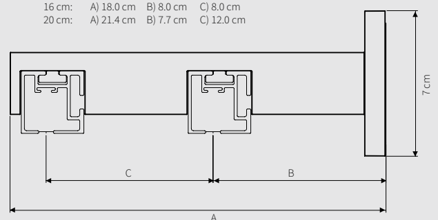
16 cm / 20 cm double wall bracket square (top fix)
