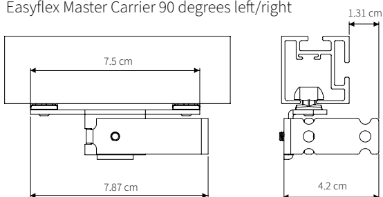
Easyflex Master Carrier 90 degrees left/right
