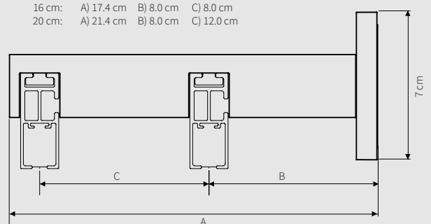
16 cm / 20 cm double wall bracket rectangular (back fix)
